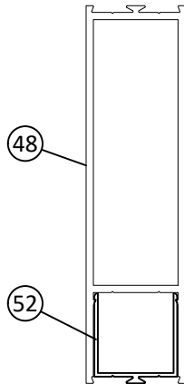
6 1/2" MID-RAIL
