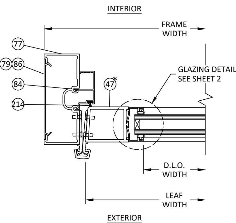
AH 14 HORIZONTAL SECTION DOOR JAMB - CONTINUOUS HINGE FG-2000 FRAMING
