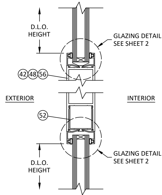
D 6 VERTICAL SECTION MID-RAIL
