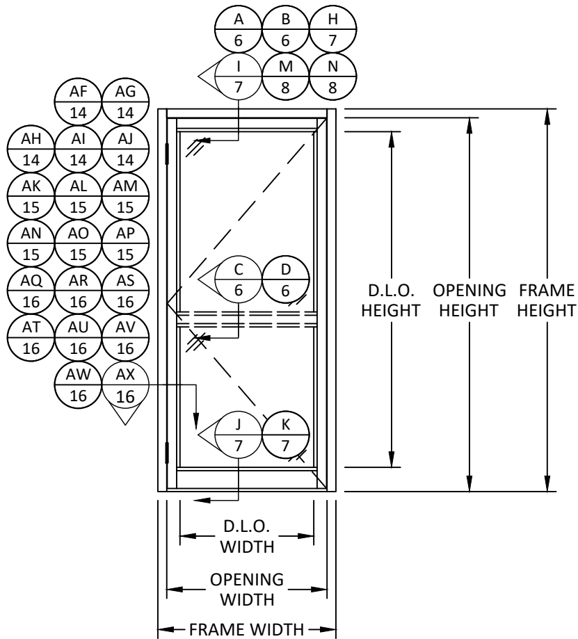
TYPICAL ELEVATION NS-212 SINGLE DOOR
