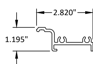
87 SHEAR BLOCK
