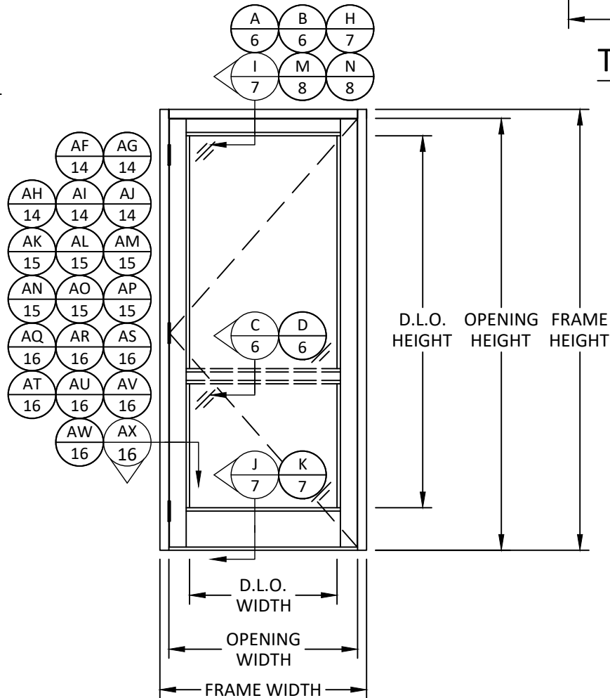
TYPICAL ELEVATION MS-375/WS-500 SINGLE DOOR
