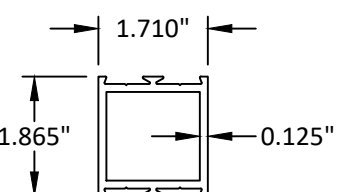
36 MID-RAIL
