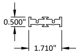
41A MID-RAIL
