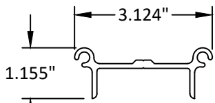
10 SHEAR BLOCK
