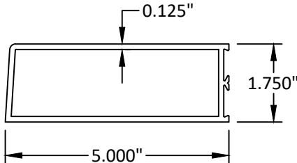
41 DOOR STILE
