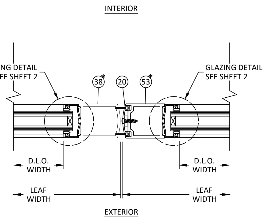
AJ 14 HORIZONTAL SECTION MEETING STILE
