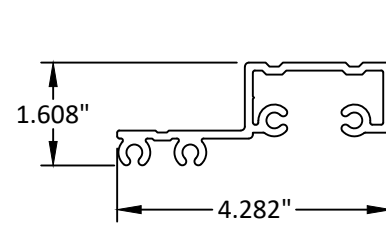
89 SHEAR BLOCK
