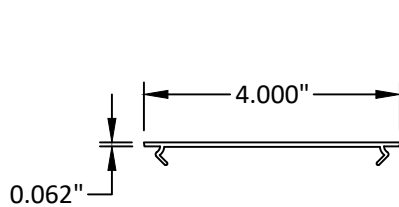
79 86 FLAT FILLER
