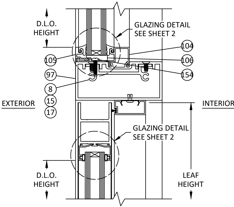
Z 11 VERTICAL SECTION DOOR HEAD W/ TRANSOM 3000 MP FRAMING - FS/BS
