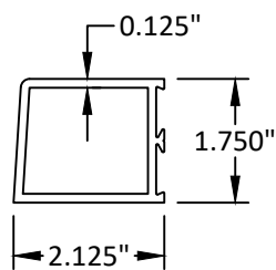
47 DOOR STILE
