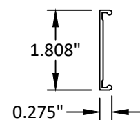
92 POCKET FILLER
