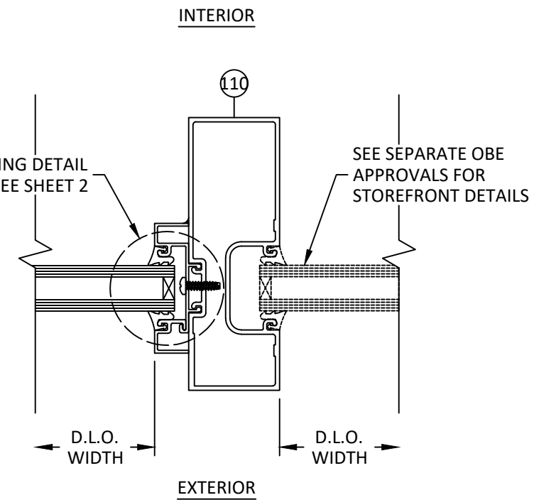
BM 18 HORIZONTAL SECTION TRANSOM JAMB W/ SIDELITE 6000 MP FRAMING - CS
