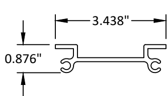
8 SHEAR BLOCK
