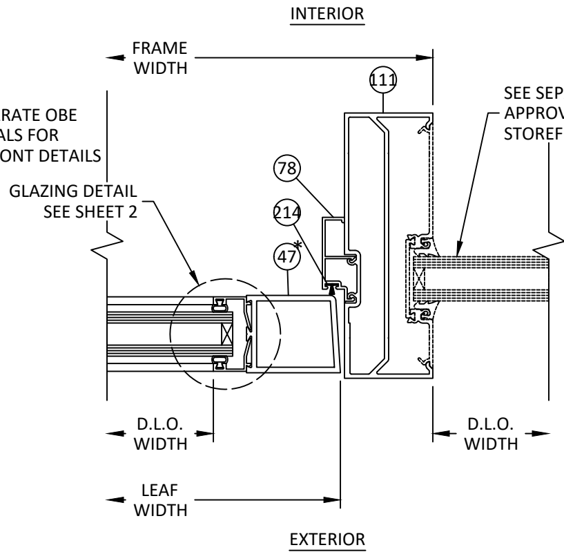
BY-21 HORIZONTAL SECTION DOOR JAMB W/ SIDELITE 6000 MP FRAMING - CS
