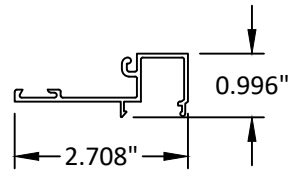
104 SASH
