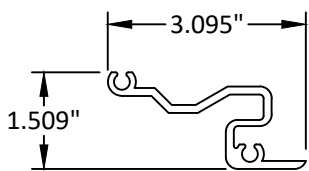
4 SHEAR BLOCK
