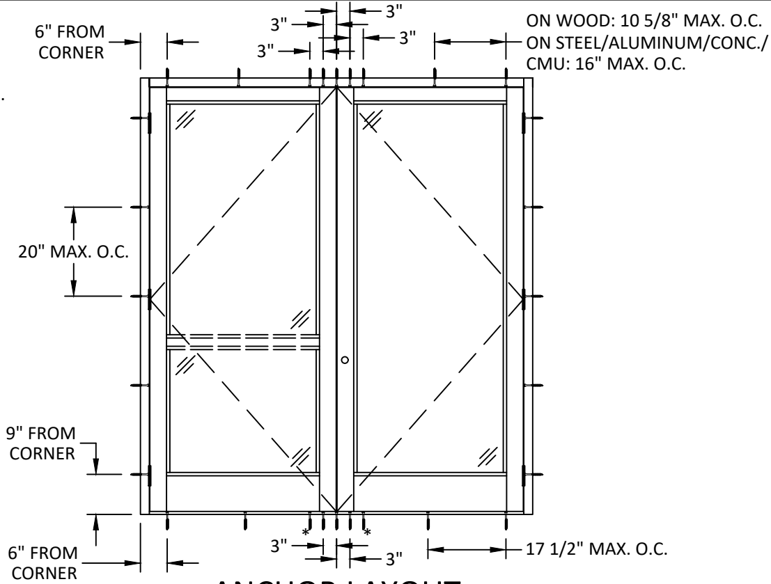
ANCHOR LAYOUT DOUBLE DOOR, DP70
