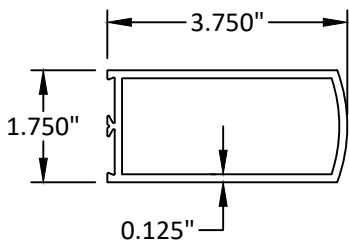
44 INACTIVE STILE
