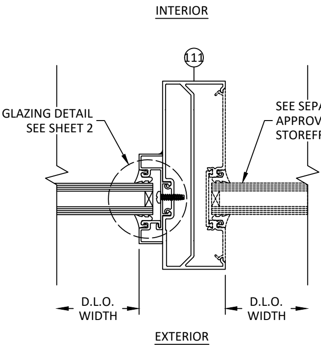
BK 18 HORIZONTAL SECTION TRANSOM JAMB W/ SIDELITE 6000 MP FRAMING - CS
