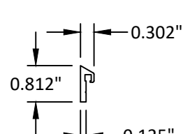
37 SWEEP RETAINER
