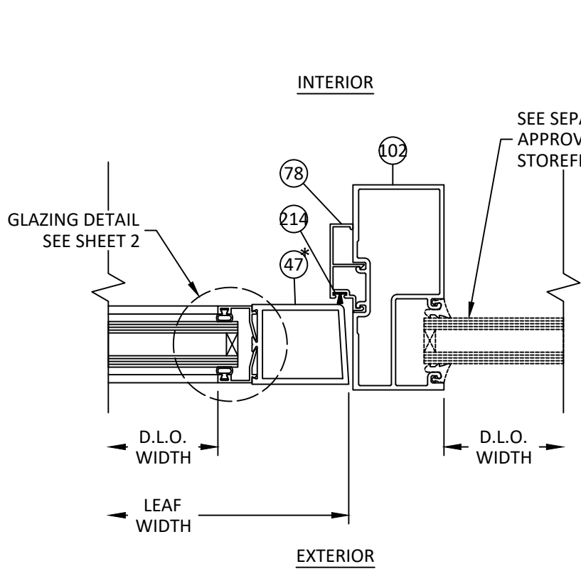
BX-21 HORIZONTAL SECTION DOOR JAMB W/ SIDELITE 3000 MP FRAMING - FS/BS
