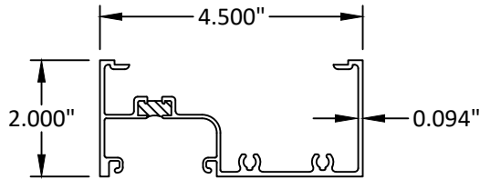
101 OPEN BACK JAMB/SILL
