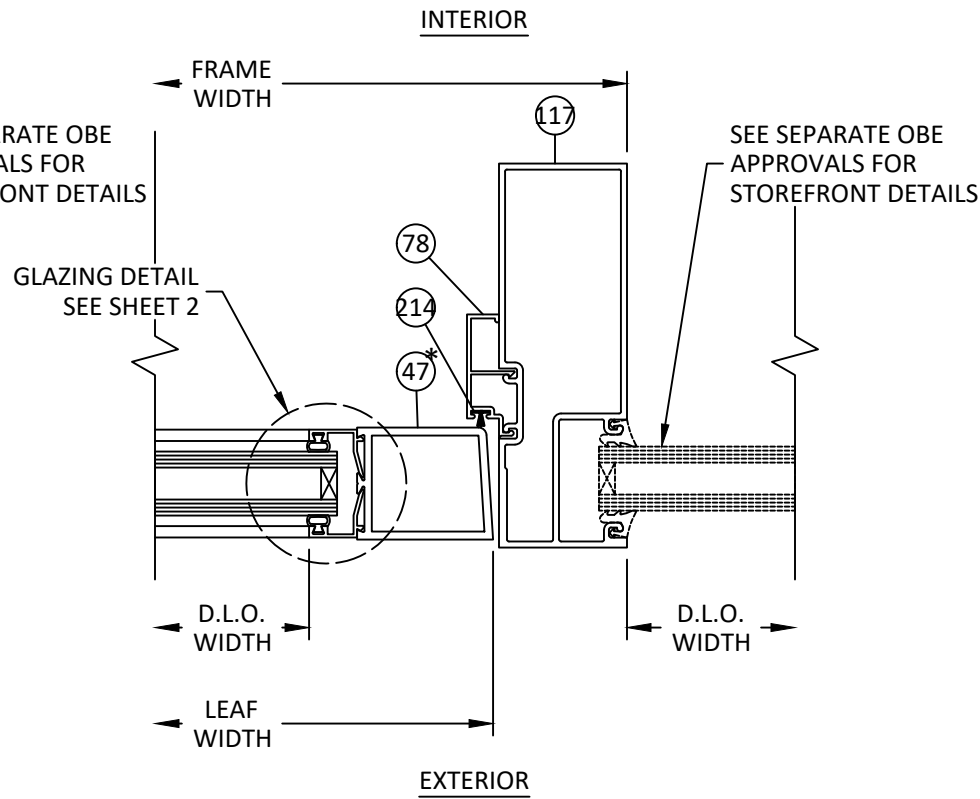
CB-21 HORIZONTAL SECTION DOOR JAMB W/ SIDELITE 6000 MP FRAMING - FS/BS
