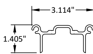
87 SHEAR BLOCK
