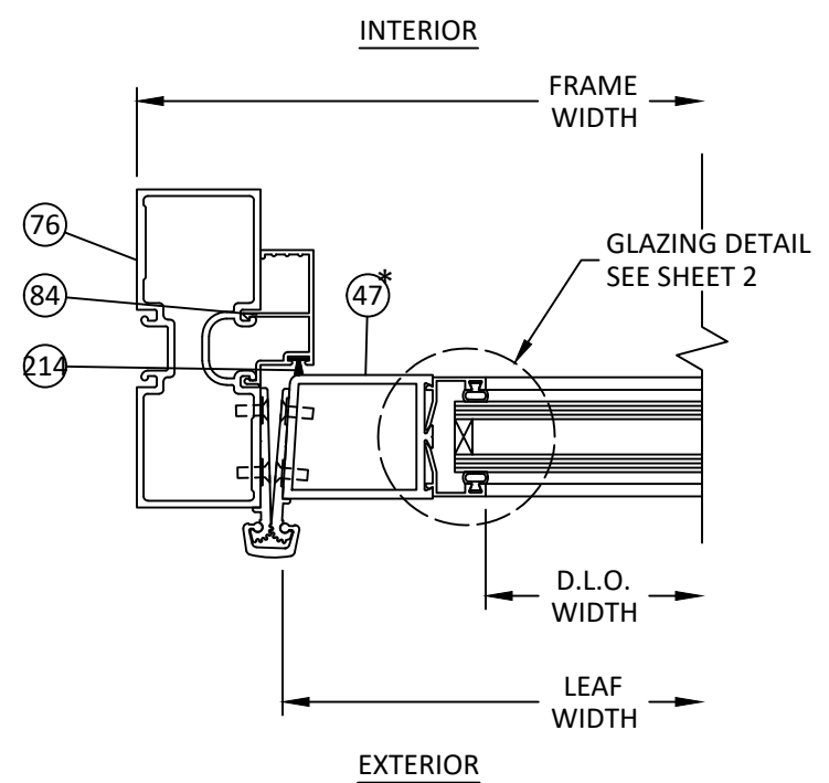
AI 14 HORIZONTAL SECTION DOOR JAMB - CONTINUOUS HINGE FG-2000 FRAMING
