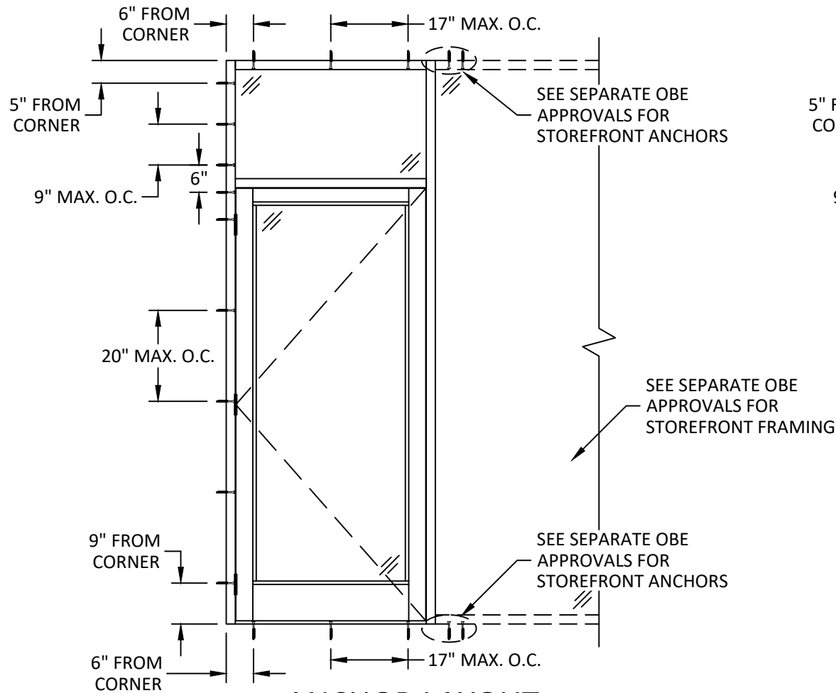
ANCHOR LAYOUT SINGLE DOOR W/ TRANSOM AND SIDELITE
