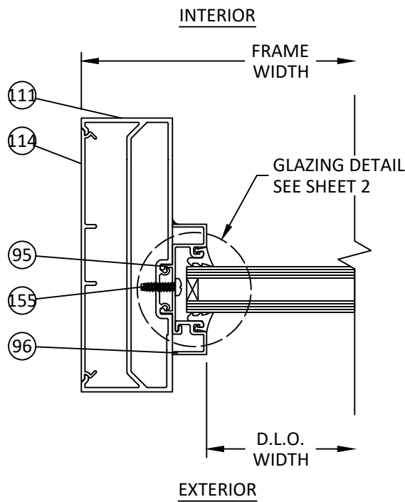
BJ 18 HORIZONTAL SECTION TRANSOM JAMB 6000 MP FRAMING - CS
