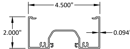
91 MULLION
