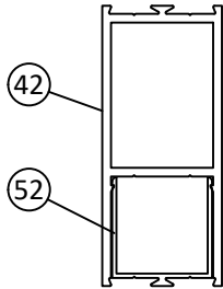
4" MID-RAIL
