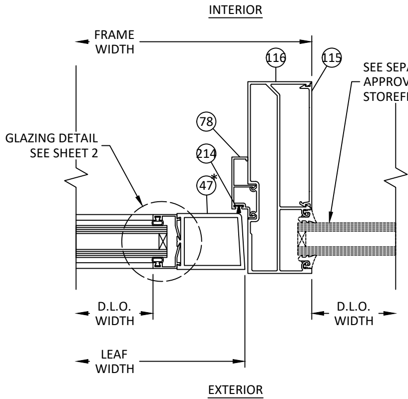
CA-21 HORIZONTAL SECTION DOOR JAMB W/ SIDELITE 6000 MP FRAMING - FS/BS
