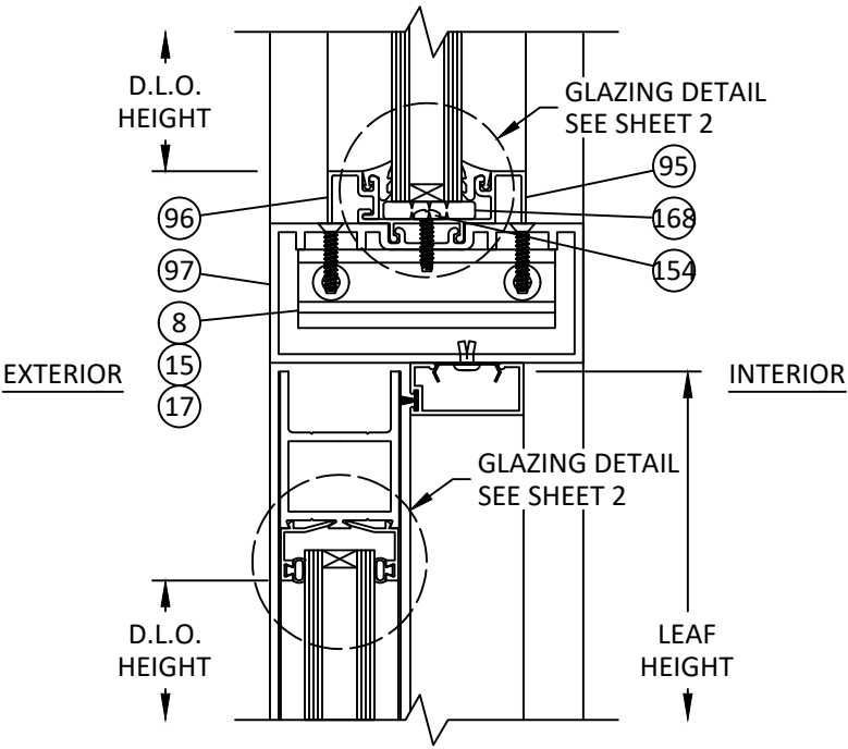
Y 11 VERTICAL SECTION DOOR HEAD W/ TRANSOM FG-3000 / 3000 MP CS FRAMING
