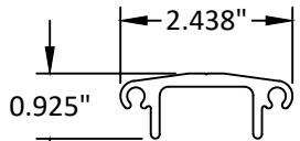
2 SHEAR BLOCK
