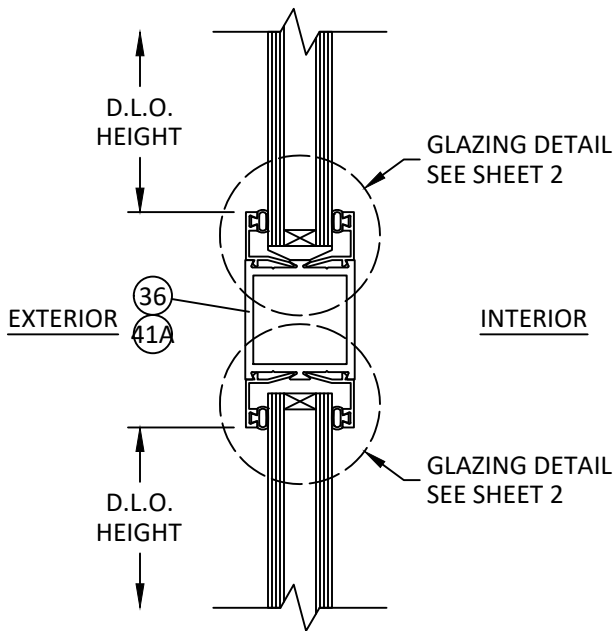
C 6 VERTICAL SECTION MID-RAIL
